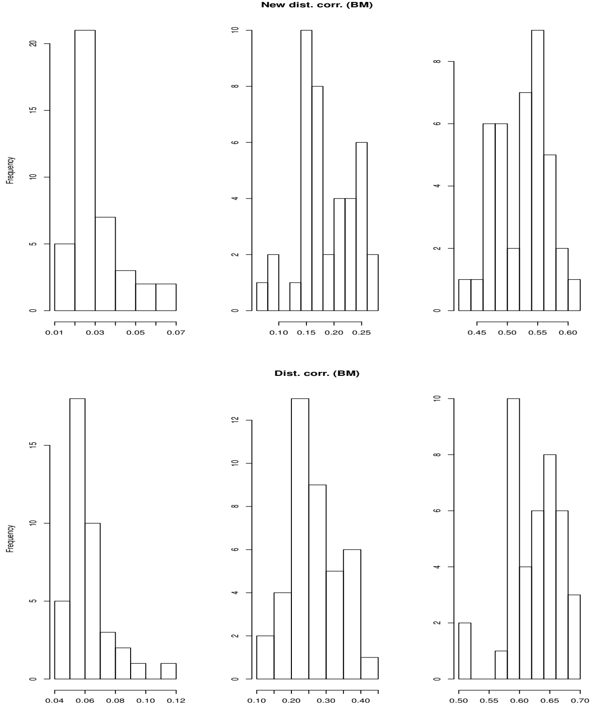
FIGURE 1. Histograms of R_n(B_1, B_2) (top) and R_n^{\text{Sz}}(B_1, B_2) (bottom) based on 40 samples. The correlations of B_1 and B_2 are respectively \rho = 0, 0.5, 0.8 , from left to right.
