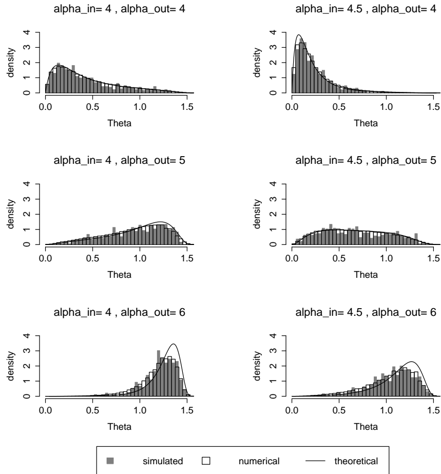
FIGURE 3. Comparison of the true angular density with estimates for various values of (\alpha_{in}, \alpha_{out}) .
