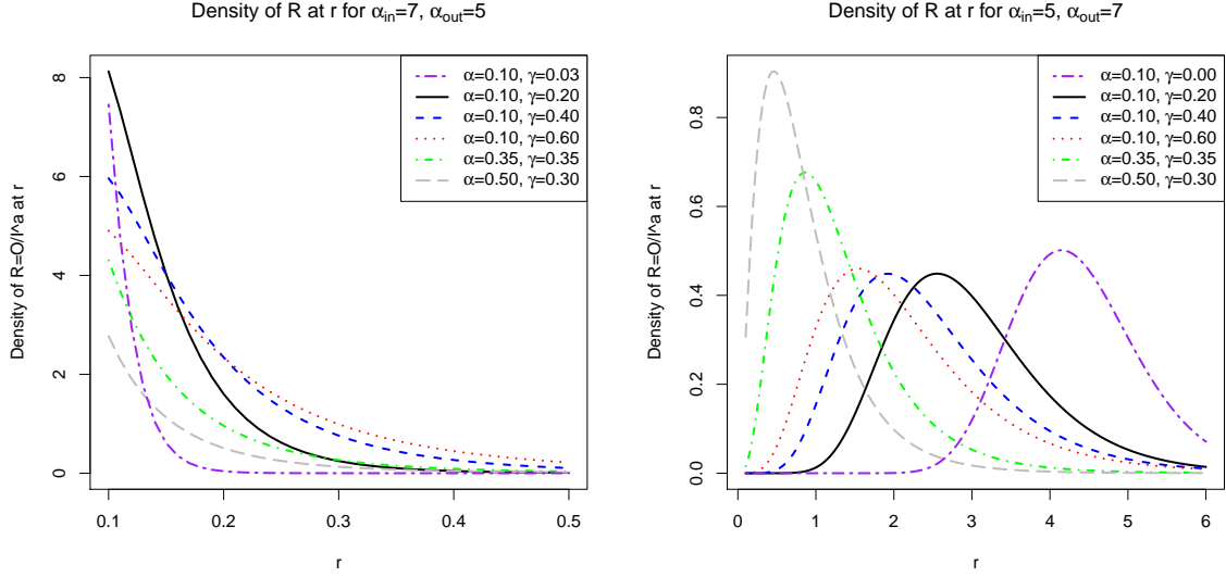
FIGURE 1. The density f_R(r) for (\alpha_{in}, \alpha_{out}) = (7, 5) (left) and (\alpha_{in}, \alpha_{out}) = (5, 7) (right) for various values of \alpha, \gamma .
