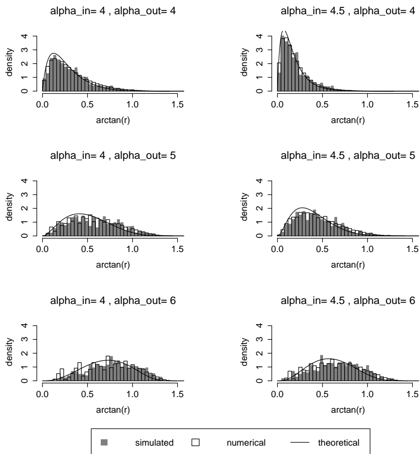
FIGURE 2. Comparison of the true density with the estimated densities of \arctan R over various values of (\alpha_{in}, \alpha_{out}) .
