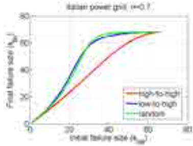
Figure 5.2: Failure cascade in Italian power grid interdependent network for a fixed threshold and three different coupling.
