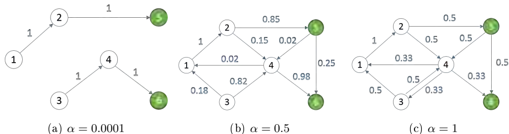
Figure 7.2: Routing continuum for target set \{5, 6\} : routing edge probabilities P^{\{5,6\}}(\alpha) for network example in Fig. (7.1a) for three different values of \alpha which generates a continuum from shortest path to all path.
