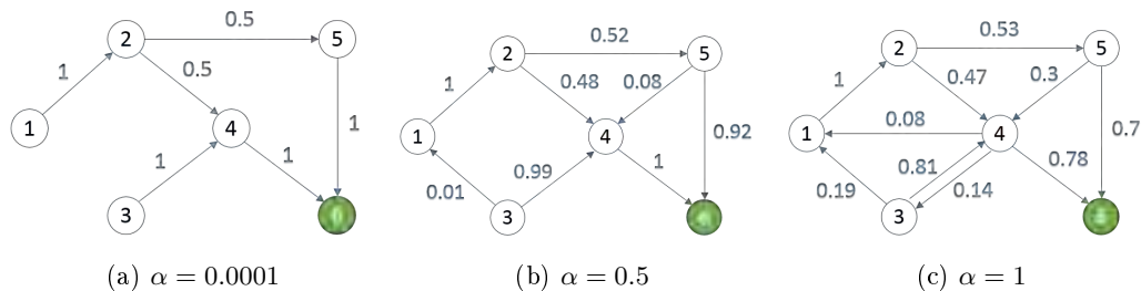
Figure 7.3: Routing continuum for logical flow: routing edge probabilities P^{\{6\}}(\alpha) for network example in fig. (7.1a) with the same edge weights but uniform edge probabilities P , for different values of \alpha which generates a continuum from shortest path to all path. Target is node 6.
